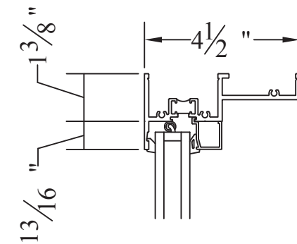
9 FIXED HEAD
