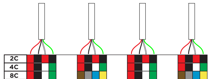
Figure 13: 4-Wires
