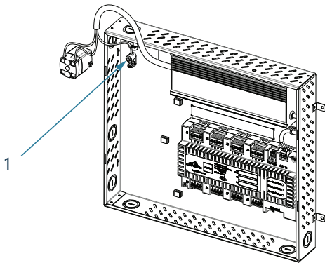
Figure 6: AC Connections
