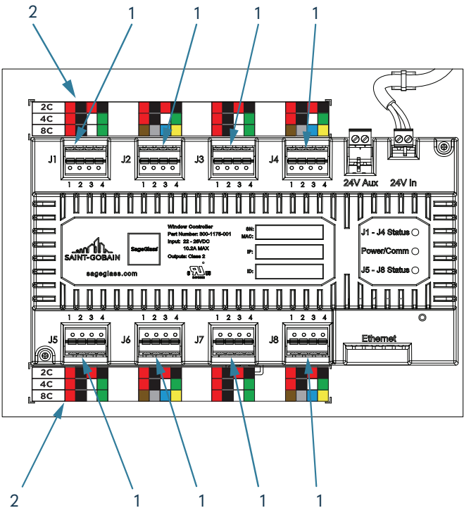
Figure 10: Controller Connection
