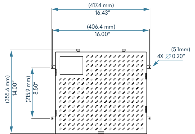
Figure 1: Installation Dimensions
