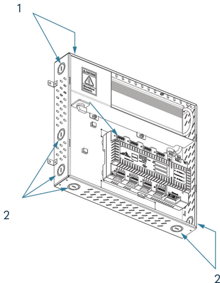
Figure 3: Knock-outs
