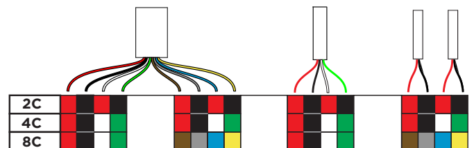
Figure 15: Mixed Wires
