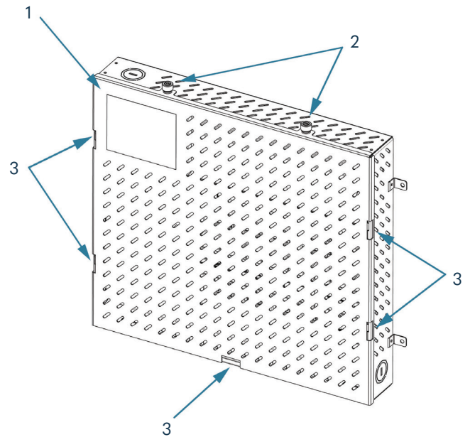
Figure 2: Cover Removal
