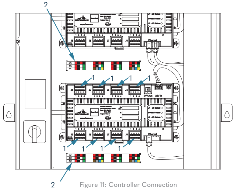
Figure 11: Controller Connection
