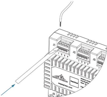
Figure 9: Terminal Connection
